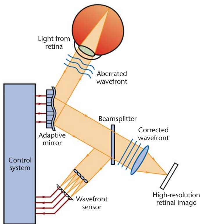
Figure 1. Schematic of an adaptive optics system. [Adapted from a figure by Chris Dainty, National University of Ireland, Galway.]
